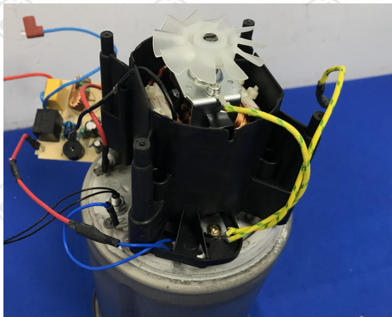
Fig.8- Internal view
