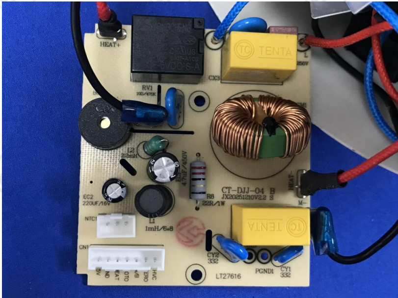
Fig.9- Main PCB
