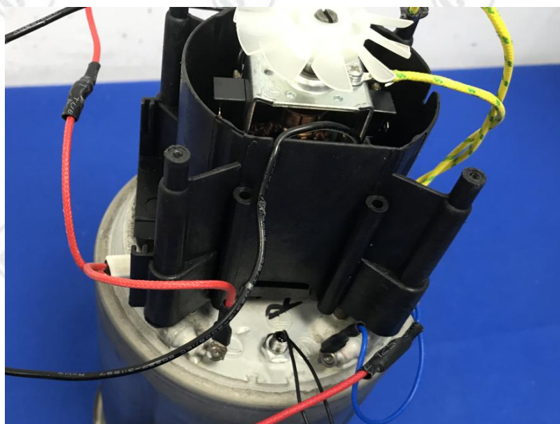
Fig.7- Internal view
